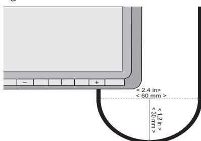
Fig. 1-6 Minimum Cable Distance
