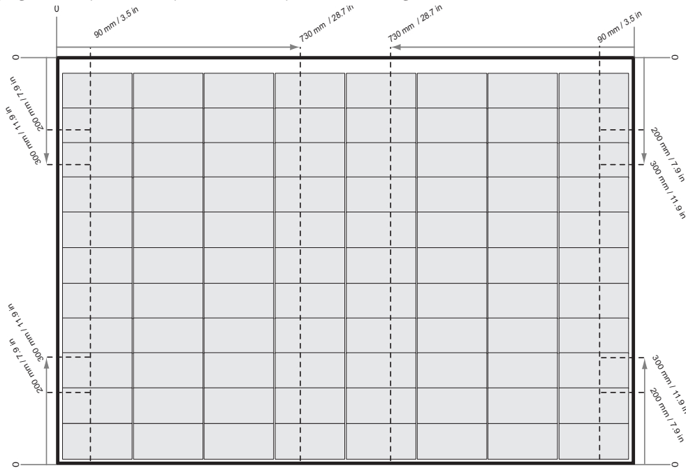
Fig. 4-2 Clamping of REC Alpha Pure-RX panels with Rails parallel to the Long Side of the Panel
