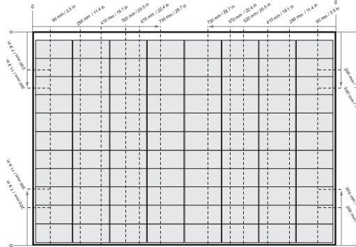
Fig. 4-3 Clamping of REC Alpha Pure-RX panels using short rails
