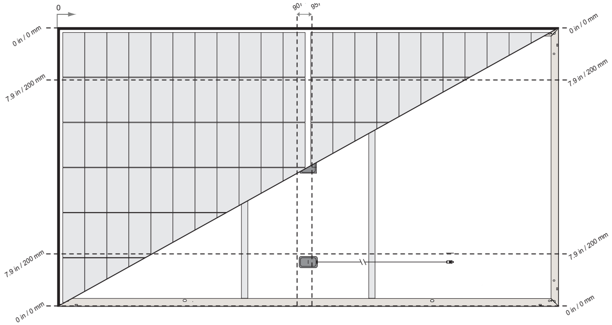
Fig. 2-5 Mixed Six-Point Mounting of REC Alpha Pure 2 Series Panels using short rails
