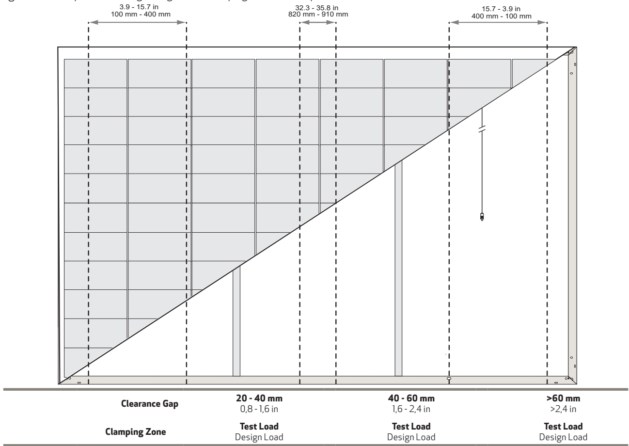
Fig. 4-4 Six-point mounting configuration clamping zones: REC Alpha Pure-RX
