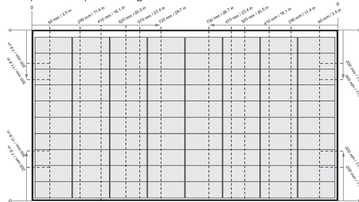
Fig. 3-3 Clamping of REC Alpha Pure-R panels using short rails
